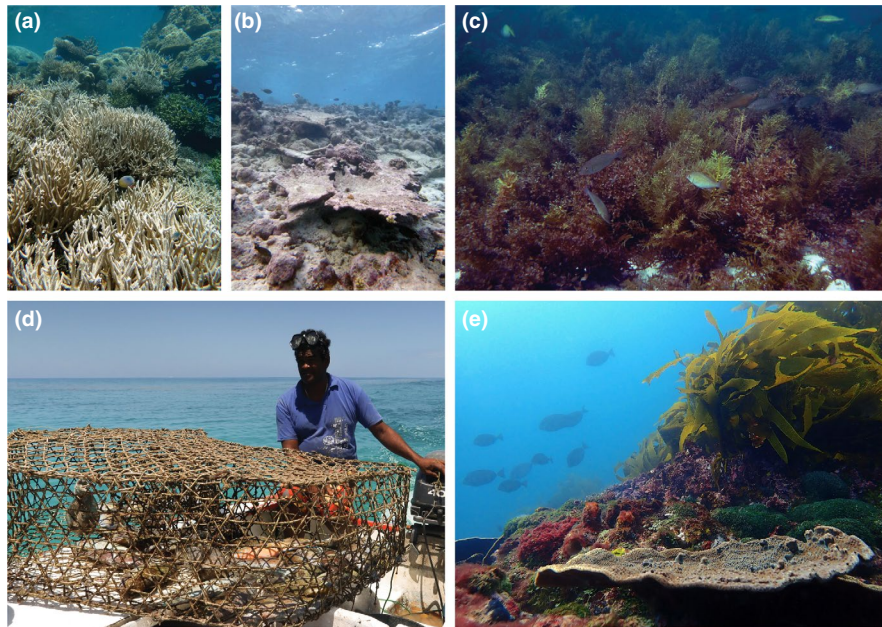
FIGURE 2 Functional shifts and novel dynamics that characterise coral reefs in the Anthropocene. Structurally complex reefs with high accretion rates and carbonate production (a) are transitioning to net-erosional states following mass coral mortality, causing a flattening of reef seascapes (b). Tropical macroalgal beds are often viewed as the negative endpoint to a coral–algal regime shift, but some species occur naturally in high abundance close to coral reefs and contribute to overall reef function. For example, tropical Sargassum beds act as important nursery habitats for juvenile reef fish (c) and can sustain productive adult fish populations and fisheries where they have replaced corals as the dominant habitat former (d). As coral reefs are being lost from some locations, in others novel reef configurations are emerging, in some cases via range extensions and the “tropicalisation” of temperate reefs that results in novel dynamics and new opportunities for human exploitation (e). Photo credits: Chris Perry (a, b), Christopher Fulton (c), James Robinson (d) and Adriana Vergés (e)
