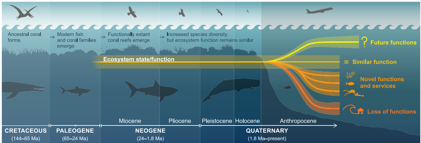
FIGURE 1 The changing scope of coral reef functional space into the Anthropocene. Functionally extant coral reefs emerged ~24 million years ago (Ma) in the early Neogene and existed in a relatively stable form prior to entering the Anthropocene. In recent decades, the scope and bounds of coral reef ecosystems have expanded and their functional future is now much more uncertain than in the geological past. For some reefs, past functions remain, and for others, key functions are being lost. As novel reef configurations form and society responds, novel functions and ecosystem services are emerging. Future reef configurations and the continued adaptation of society will likely result in functions we have not yet seen or recognised as important
