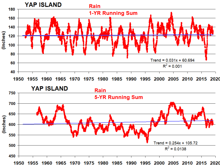
Figure Y3. The Post-WWII historical record of rainfall at WSO Yap Island. Top panel is a 12-month running sum of rainfall, and the bottom panel is a 5-year running sum. Note the high variability of the 12-month rainfall that is in large measure an effect of ENSO. The 5-year running sum brings out longer-period variability, with the dry decade of the late 1980s-to-early 1990s and the wet decade of the 2000s sharply apparent. The long-term trend of each time series (blue lines) show a modest rising trend of .03 inches per year for the 1-year sum, and .25 inches per 5-year block for the 5-year sum (the 5-year sum slightly exaggerates the small trend seen in the 1-year running summation).
