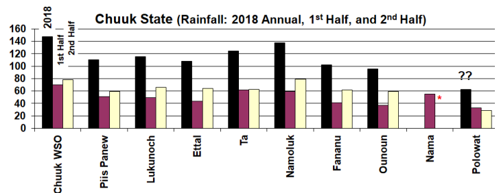
Figure CH-2. A bar chart depiction of 2018 rainfall totals at the indicated locations within Chuuk State. The black bar shows the 2018 annual total; the maroon bar shows the 2018 1 st half total; and, the yellow bar shows the 2018 2 nd half total. Only the 1 st half total was available for Nama Atoll. Polowat almost always is much drier than at the other locations; this might indicate an exposure problem with the rain gauge.
