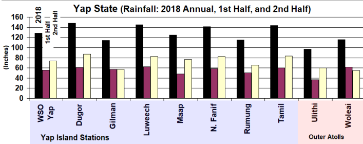
Figure Y2. A medley of rainfall amounts at locations within Yap State. The three bars for each location indicate the 2018 annual, 2018 1 st half, and 2018 2 nd half rainfall totals, respectively. Locations in the blue shading are on Yap Island, and the locations in the light red shading are two of the State’s outer atolls. The annual average rainfall at WSO Yap is about 120 inches.
