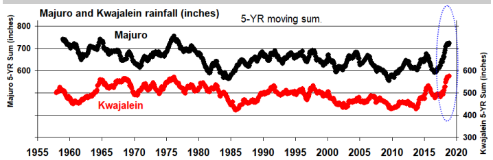
Figure RMI-2. 1- and 5-year moving sums of accumulated rainfall at (a) Kwajalein and (b) Majuro (looking backwards). Note two features of these time series: the long-term downward trend and the abrupt upswing at the end of each time series. Chart (c) is a juxtaposition of the 5-year rainfall sum at Kwajalein and Majuro illustrating a notable similarity of rainfall behavior. Note that by July 2018 the Kwajalein 5-year sum had risen to its highest value in its historical record. Note that prior to the current “spike” of heavy rainfall, Majuro and Kwajalein had undergone a continual decline in rainfall over the span of their post-WWII historical record (blue dotted lines).
